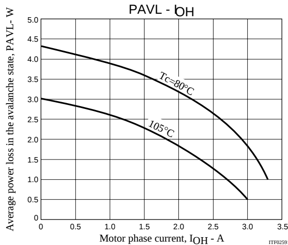
Figure 3 Allowable Loss Range, PAVL-I_{OH} During STK672-640A-E Avalanche Operations
