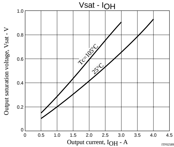
STK672-640A-E Output saturation voltage, V_{sat} - Output current, I_{OH}
