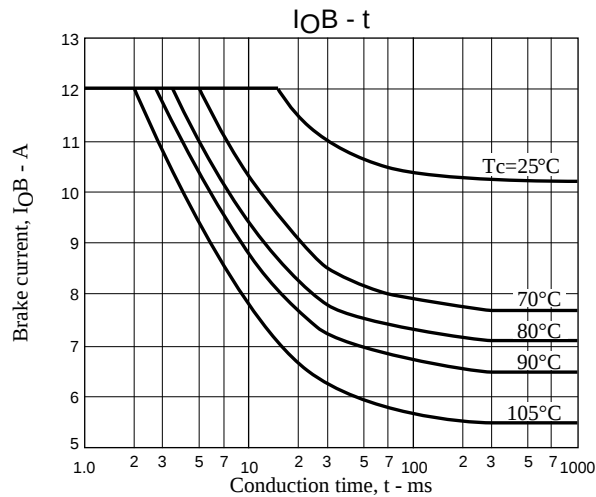
STK681-352-E Allowable Brake Current Range (Low side: F3, F4=ON)
