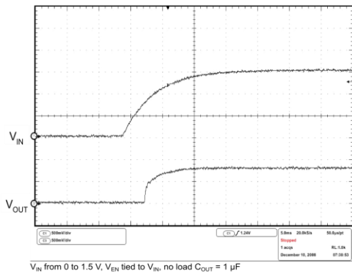
Figure 16: Start-up transient
