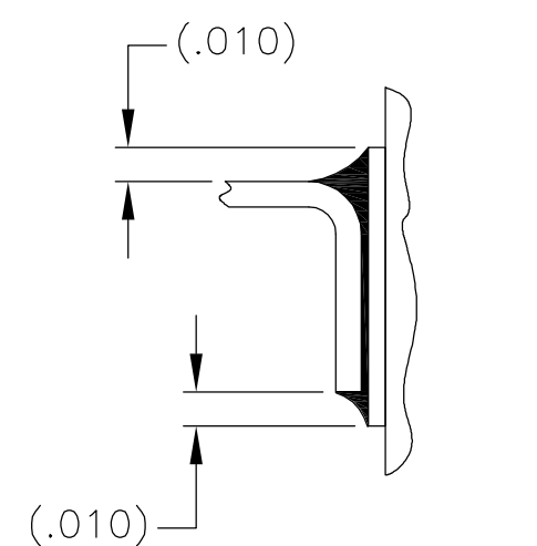
TYPICAL FOOT PLACEMENT ON SOLDER PAD
