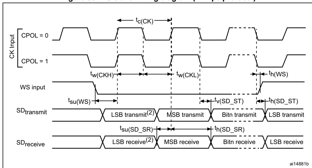
Figure 30. I2S slave timing diagram (Philips protocol)
