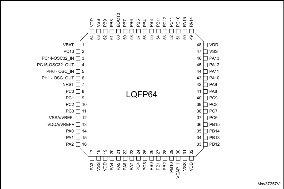
Figure 6. LQFP64 pinout
