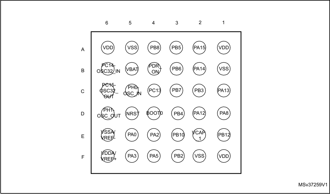
Figure 7. WLCSP36 pinout
