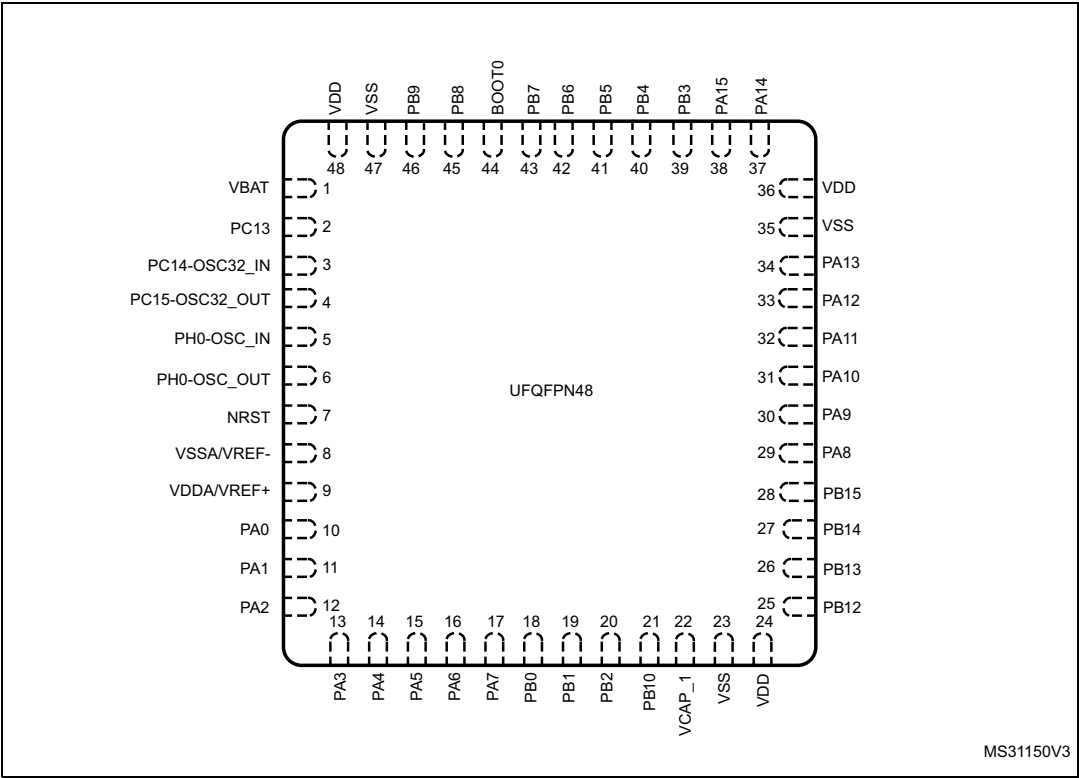
Figure 6. UFQFPN48 pinout
