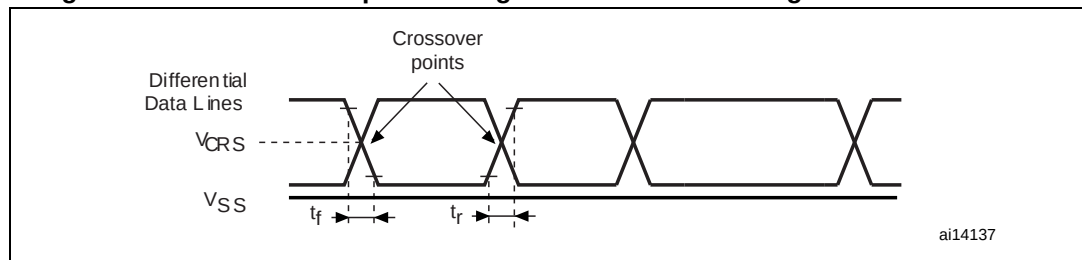
Figure 49. USB OTG full speed timings: definition of data signal rise and fall time
