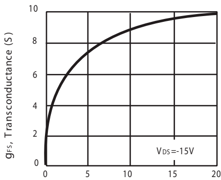
Figure 7. Transconductance Variation with Drain Current
