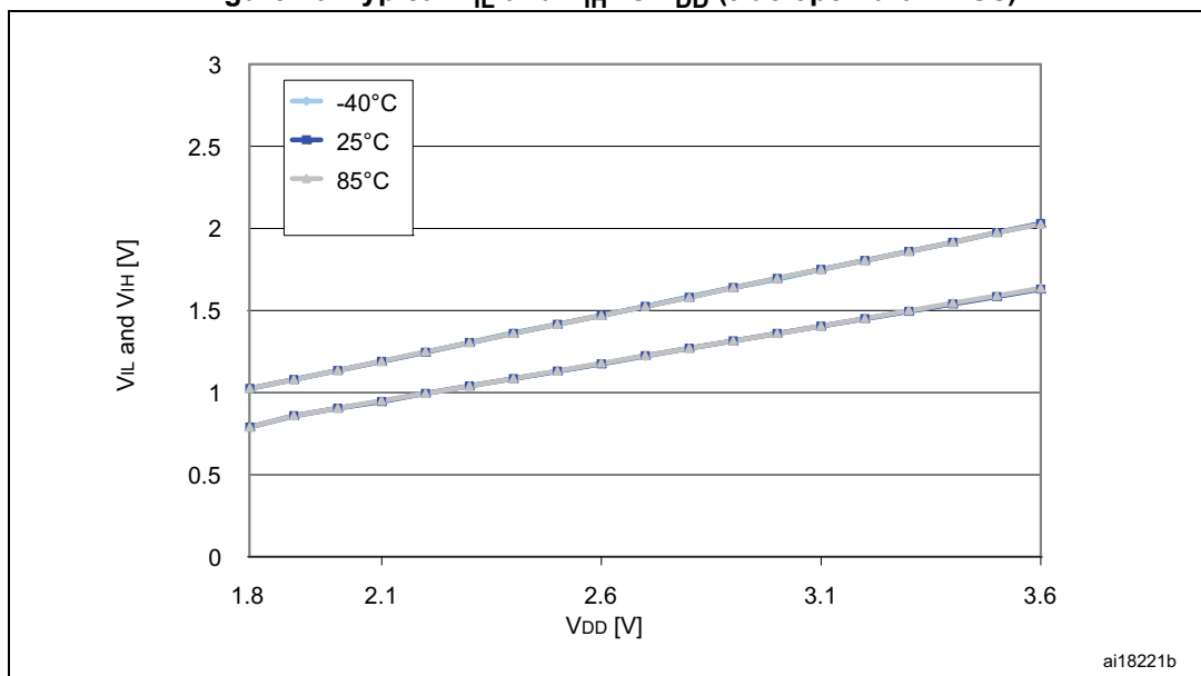
Figure 20. Typical V_{IL} and V_{IH} vs V_{DD} (true open drain I/Os)
