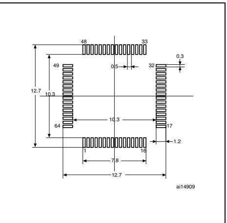
Figure 44. Recommended footprint (1)(2)
