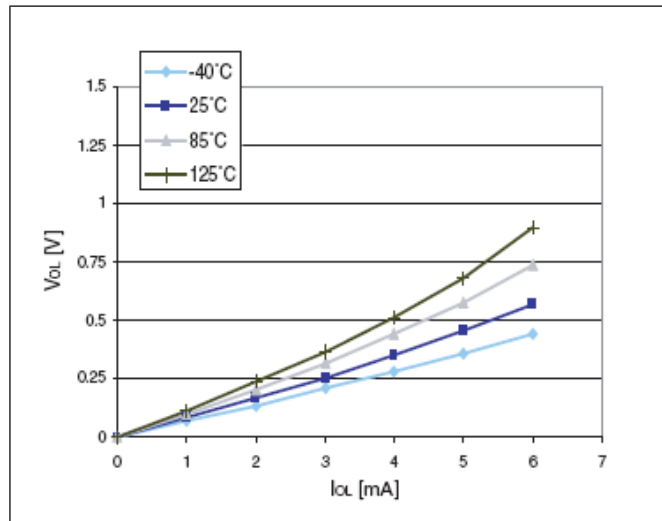
Figure 28: Typ. V_{OL} @ V_{DD} = 3.3 V (standard ports)
