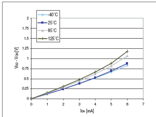
Figure 34: Typ. V_{DD} - V_{OH} @ V_{DD} = 3.3 V (standard ports)
