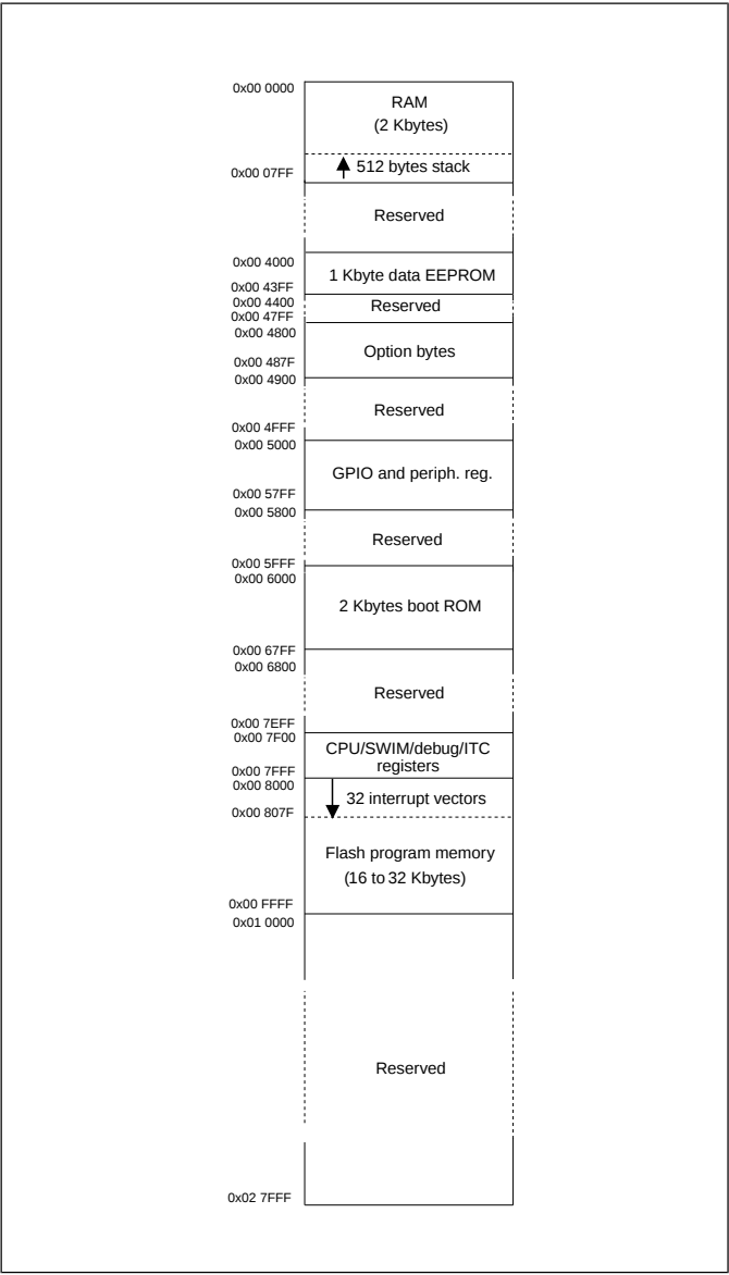
Figure 7: Memory map
