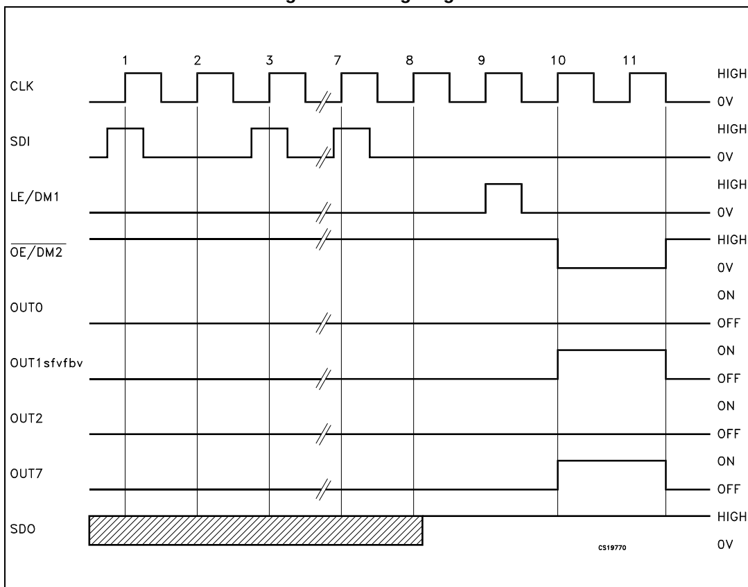
Figure 7. Timing diagram
