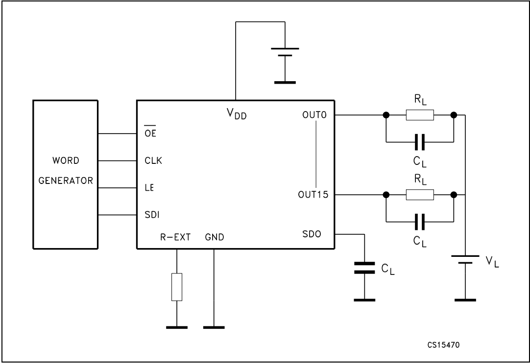
Figure 16. AC characteristics
