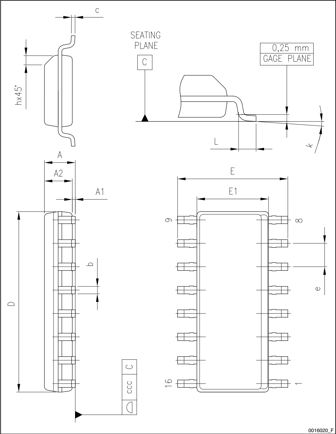
Figure 21. Package drawing
