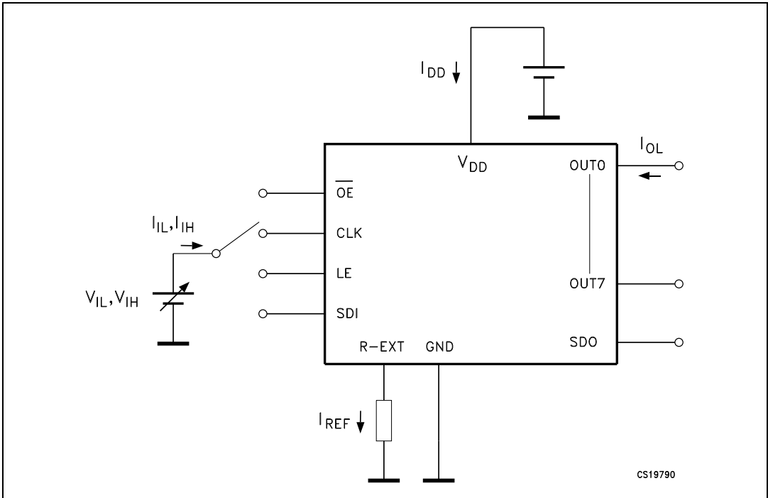
Figure 15. DC characteristics
