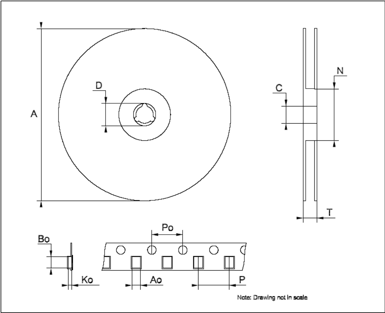
Figure 19. Reel dimensions
