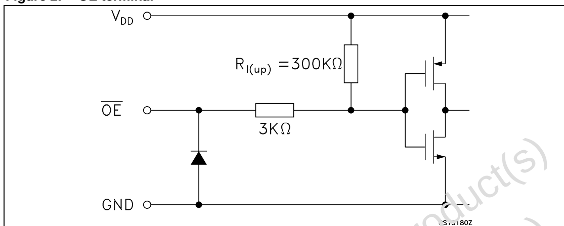
Figure 2. \overline{\text{OE}} terminal
