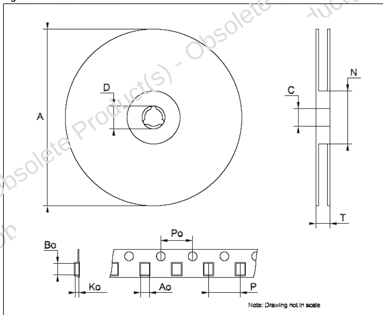
Figure 21. Reel dimensions
