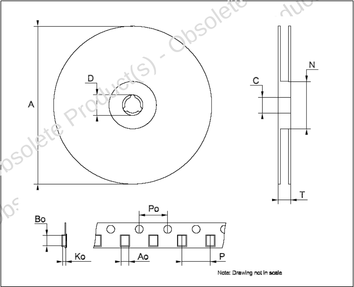
Figure 20. Reel dimensions
