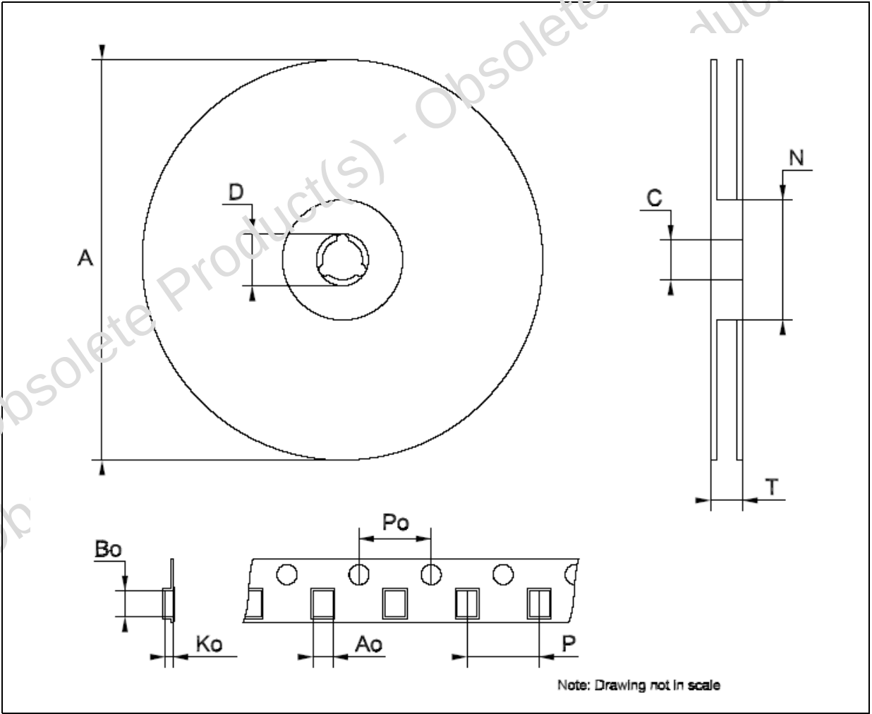
Figure 22. Reel dimensions
