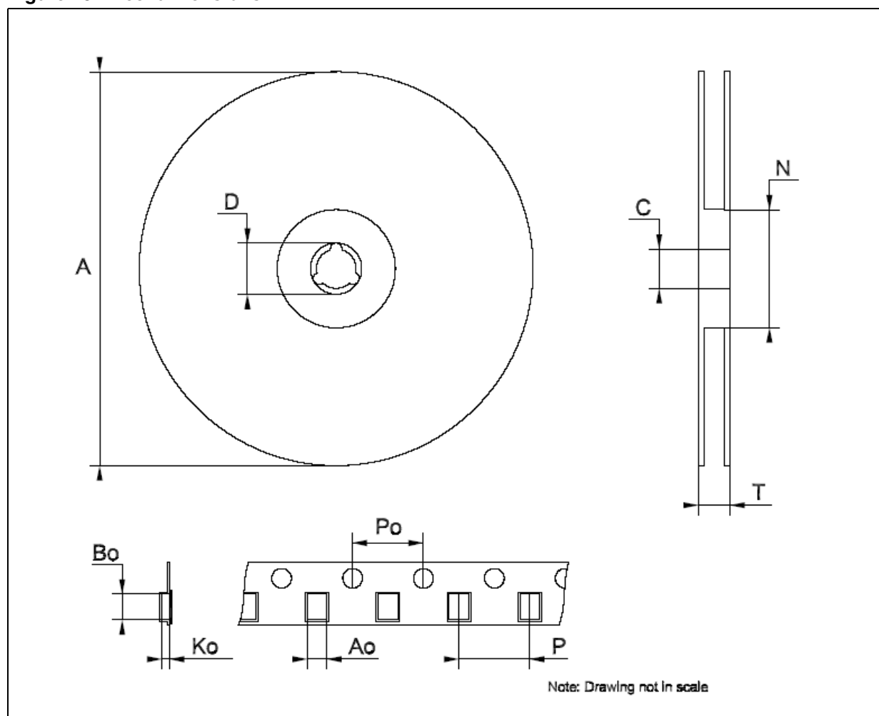
Figure 20. Reel dimensions
