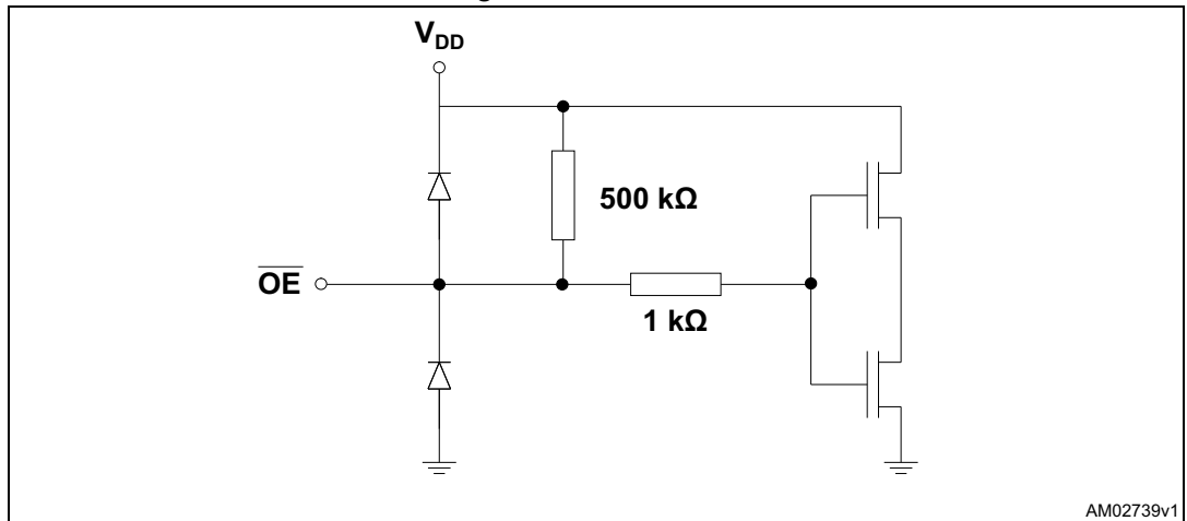
Figure 4. \overline{\text{OE}} terminal
