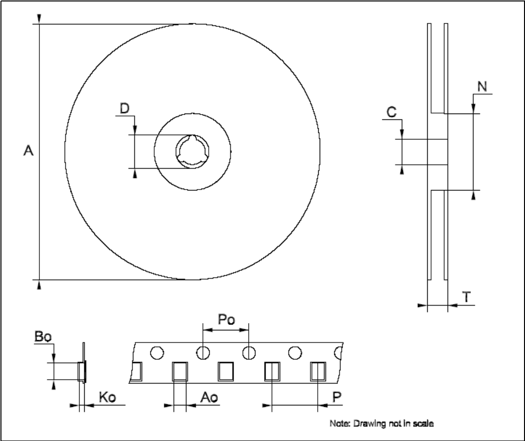
Figure 22. TSSOP-24 and TSSOP-24 exposed pad tape and reel dimensions
