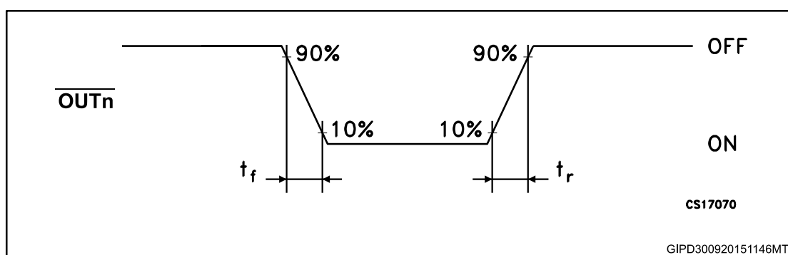
Figure 10: Outputs
