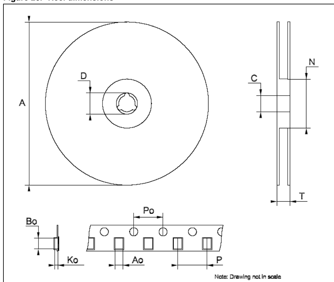
Figure 26. Reel dimensions
