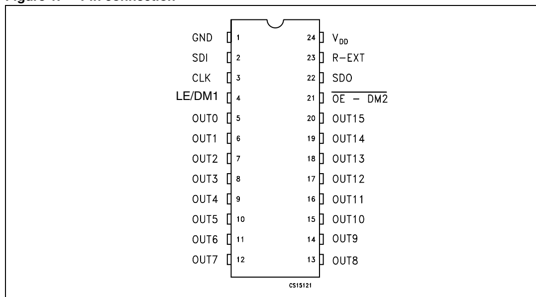
Figure 1. Pin connection
