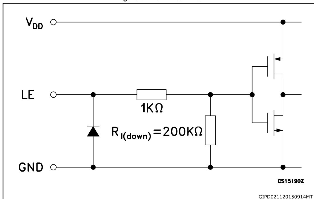
Figure 3: LE/DM1 terminal
