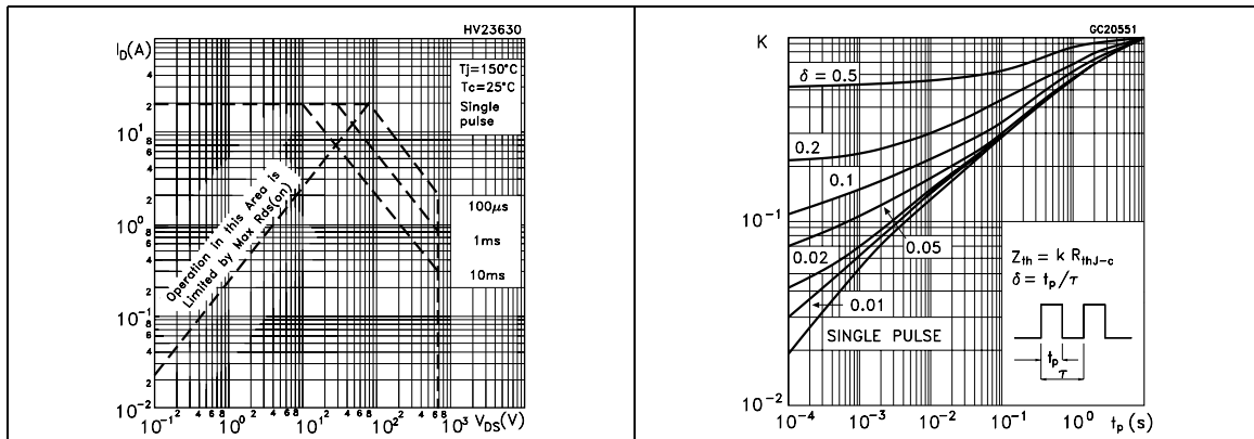
Figure 5. Safe operating area for TO-247
