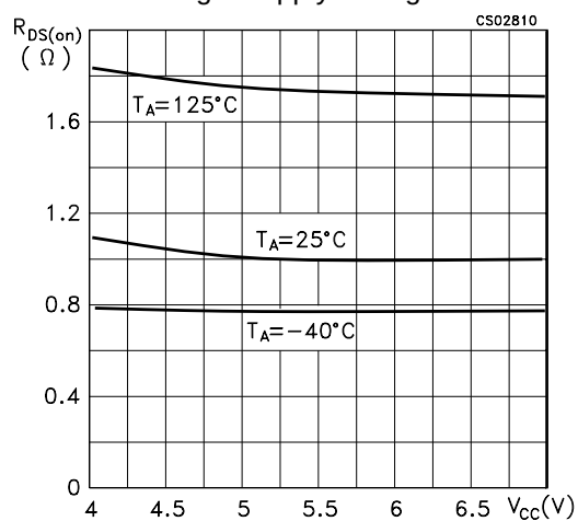
Figure 5 : Chopping Mode Characteristics
