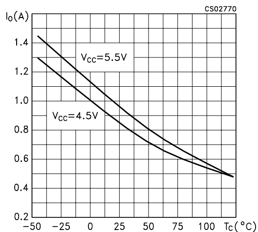
Figure 6 : Output Current vs Case Temperature
