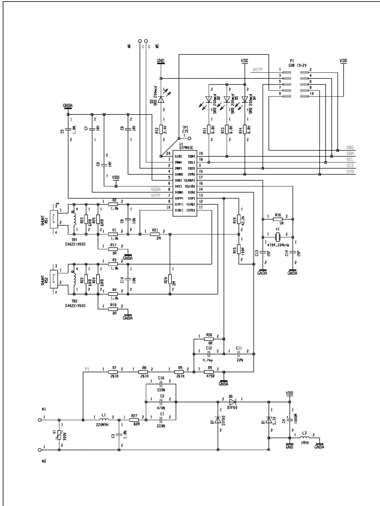
Figure 24. Application schematic
