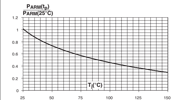
Figure 4. Normalized avalanche power derating versus junction temperature
