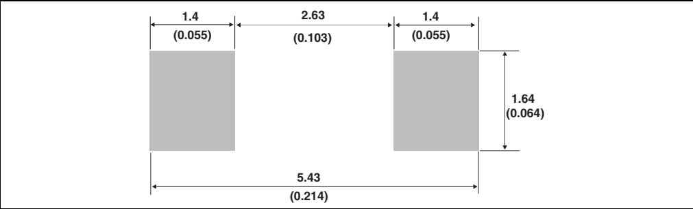
Figure 14. Footprint, dimensions in mm (inches)
