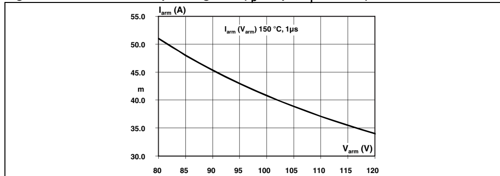
Figure 12. Reverse safe operating area ( t_p < 1 \mu s , T_j < 150^\circ C )
