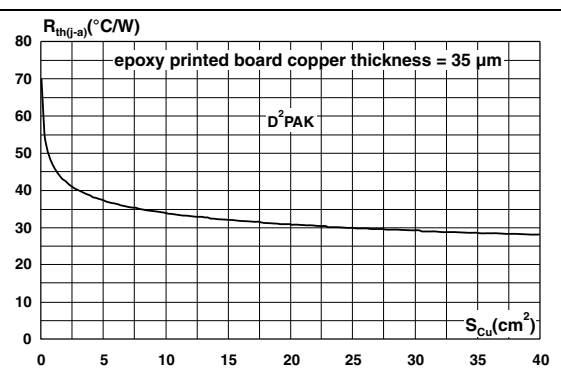
Figure 11. Thermal resistance junction to ambient versus copper surface area under tab
