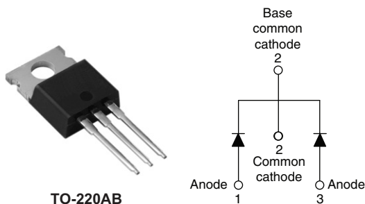
TO-220AB
