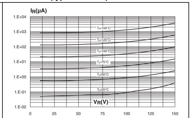
Figure 12. Reverse leakage current versus reverse voltage applied (typical values)
