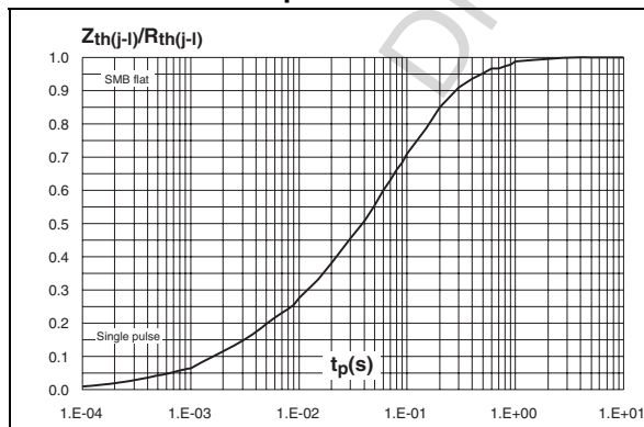
Figure 11. Relative variation of thermal impedance junction to lead versus pulse duration
