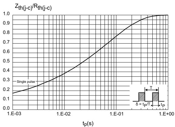
Figure 5. Relative variation of thermal impedance junction to case versus pulse duration (DPAK)
