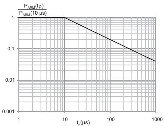
Figure 4. Normalized avalanche power derating versus pulse duration ( T_j = 125\text{ °C} )
