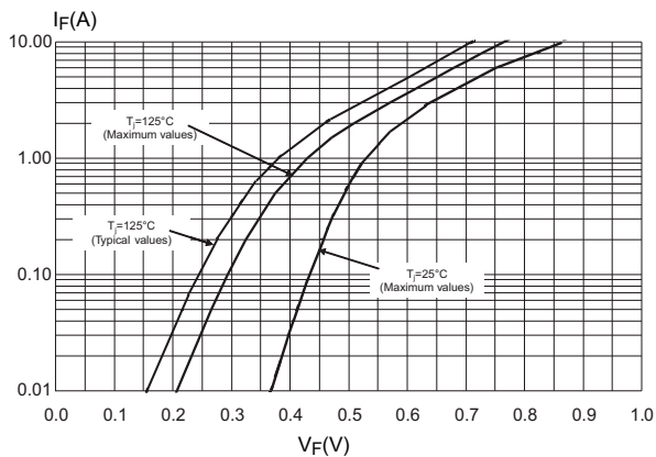
Figure 11. Forward voltage drop vs. forward current
