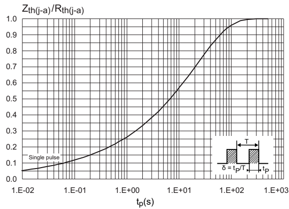
Figure 7. Relative variation of thermal impedance junction to ambient versus pulse duration (SMC)
