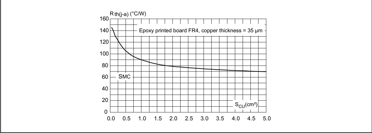
Figure 15. Thermal resistance junction to ambient versus copper surface under each lead
