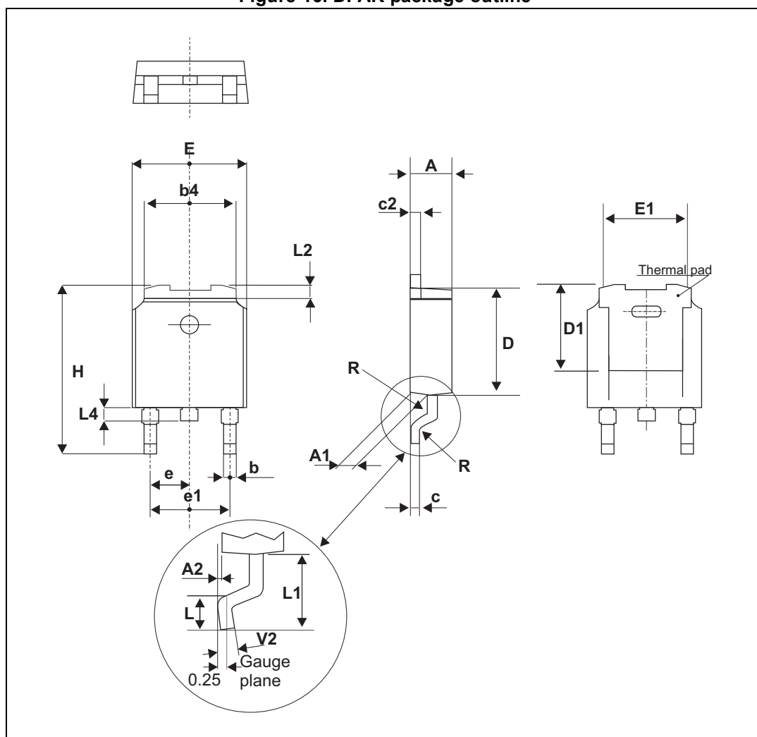
Figure 16. DPAK package outline
