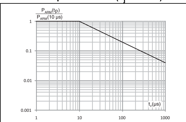
Figure 4. Normalized avalanche power derating versus pulse duration ( T_j = 125^\circ\text{C} )
