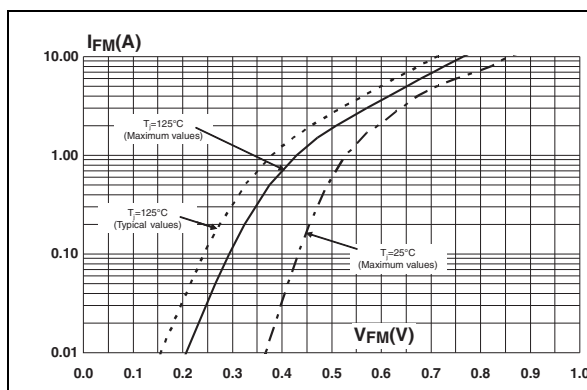
Figure 11. Forward voltage drop vs. forward current
