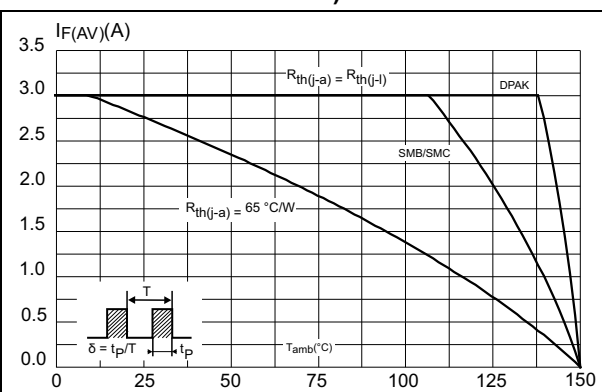
Figure 2. Average forward current versus ambient temperature ( \delta = 0.5 ) (DPAK, SMB, SMC)
