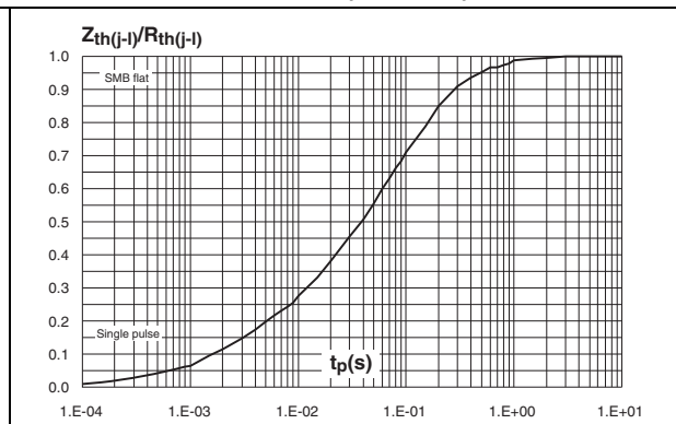
Figure 8. Relative variation of thermal impedance junction to lead versus pulse duration (SMBflat)
