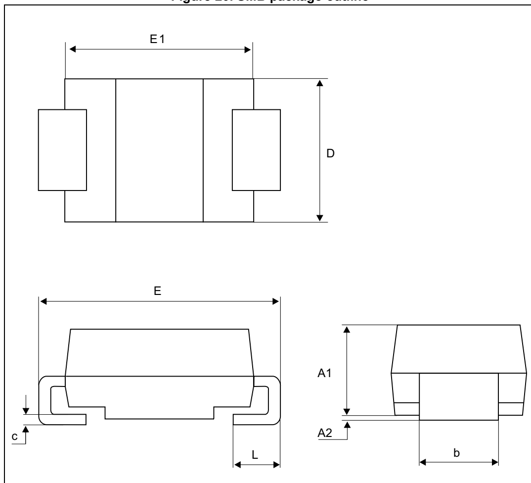
Figure 20. SMB package outline
