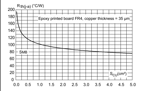
Figure 15. Thermal resistance junction to ambient versus copper surface under each lead
