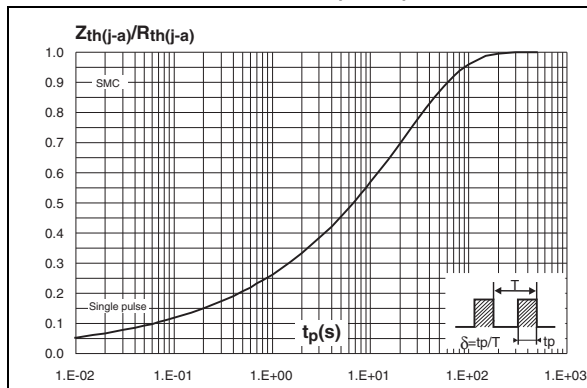
Figure 7. Relative variation of thermal impedance junction to ambient versus pulse duration (SMC)
