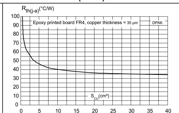
Figure 12. Thermal resistance junction to ambient versus copper surface under each lead (DPAK)
