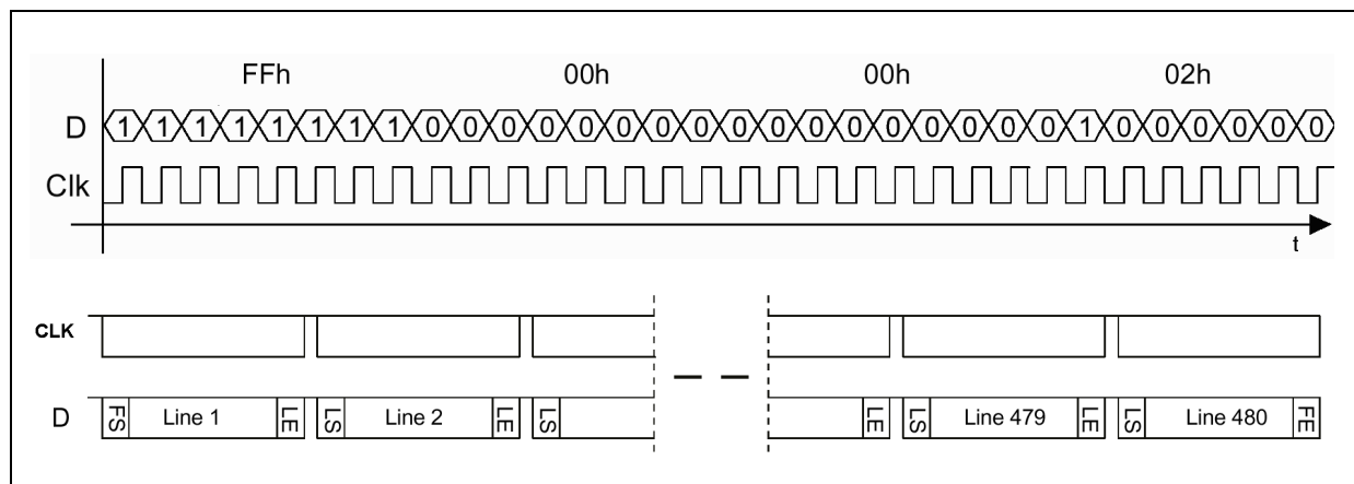
Figure 12. Bit order in synchronization codes and data, LSB first (example start of frame), image frame structure
