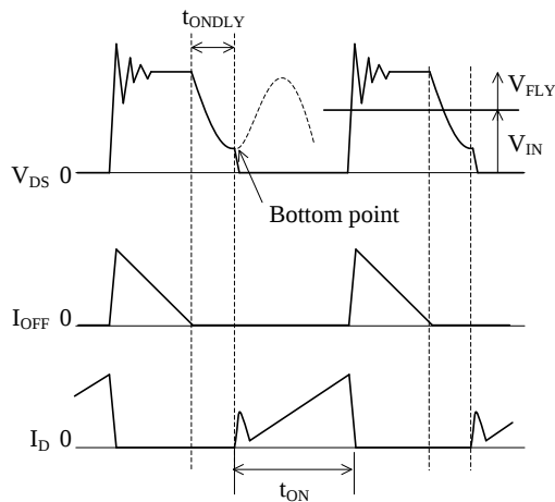
Figure 9-9 Ideal bottom-on operation waveform
