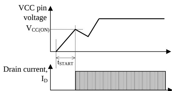
Figure 9-2 Startup operation
