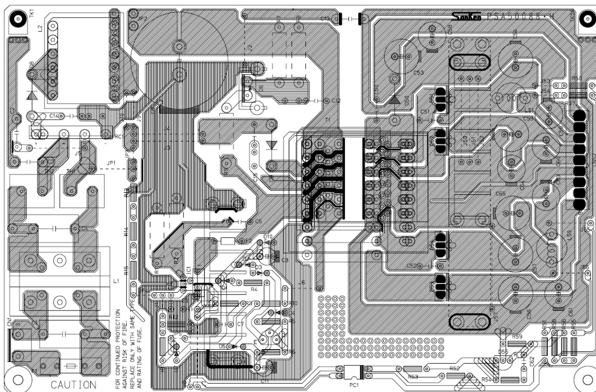
Figure 11-1 PCB circuit trace layout example
