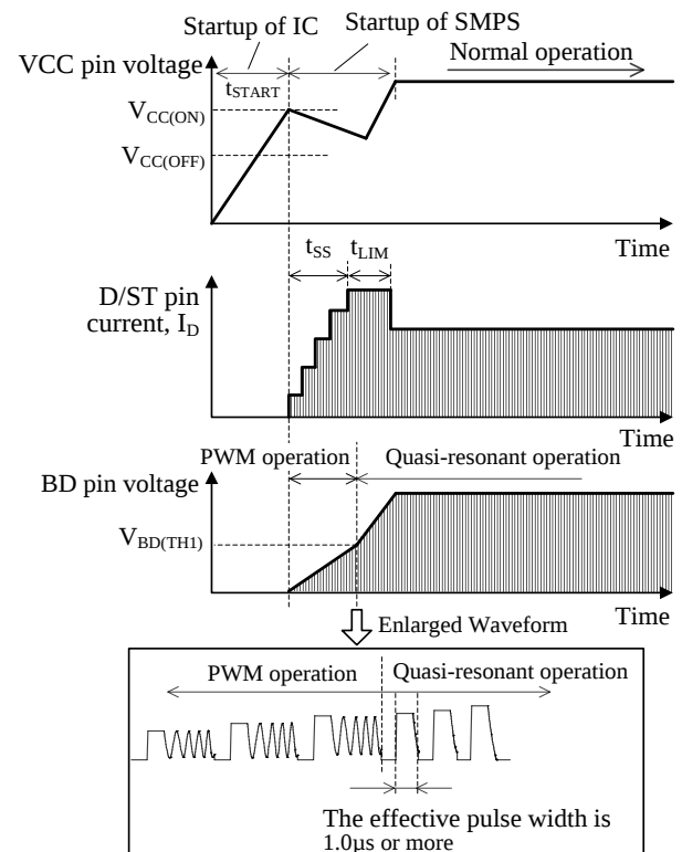
Figure 9-5 V_{CC} and I_D and V_{BD} behavior during startup
