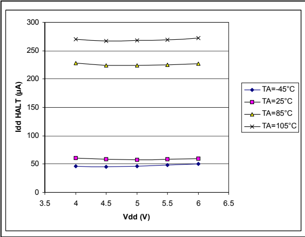
Figure 9. HALT I_{DD} vs. V_{DD}
