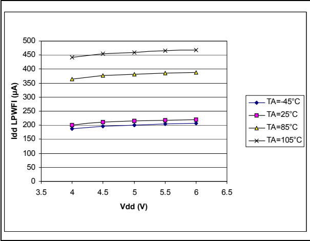
Figure 11. LPWFI I_{DD} vs. V_{DD}
