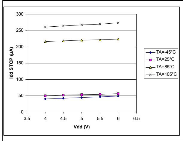
Figure 8. STOP I_{DD} vs. V_{DD}
