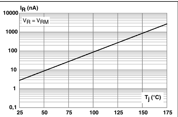
Figure 15. Leakage current versus junction temperature (typical values) STRVSxxxE
