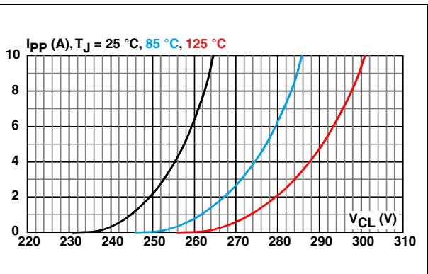
Figure 11. Clamping voltage versus peak pulse current - STRVS280X02F
