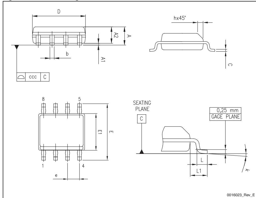
Figure 19. SO-8 drawing
