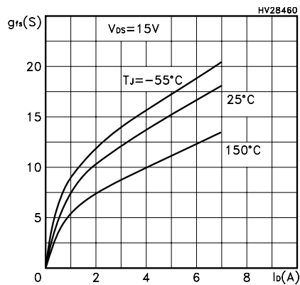
Figure 5. Transconductance
