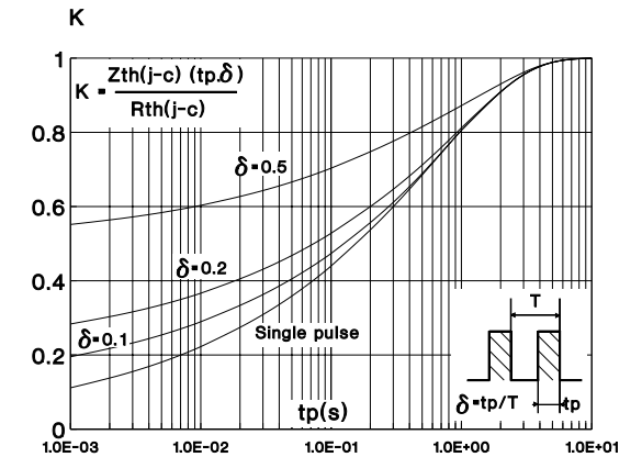
Fig. 10: Relative variation of thermal transient impedance junction to case versus pulse duration (ISOWATT220AC).
