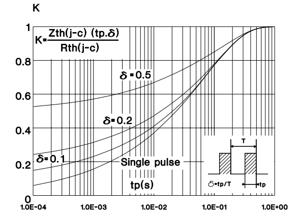
Fig. 9: Relative variation of thermal transient impedance junction to case versus pulse duration (TO-220AC and DPAK).
