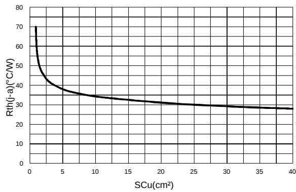
Figure 11: Thermal resistance, junction to ambient, versus copper surface under tab (epoxy printed board FR4, eCu = 35μm) (D 2 PAK)
