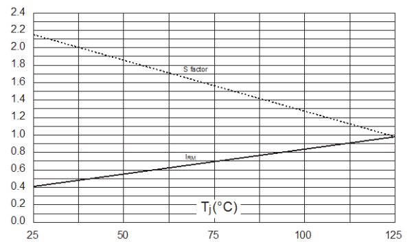
Figure 8: Relative variation of dynamic parameters versus junction temperature (reference: T_J = 125^\circ\text{C} )
