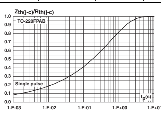
Figure 4. Relative variation of thermal impedance junction to case versus pulse duration (TO-220FPAB)
