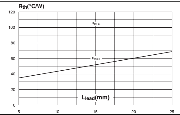
Figure 12. Thermal resistance versus lead length (DO-41)
