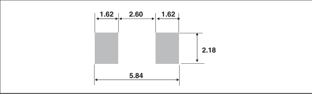
Figure 14. Footprint (dimensions in mm)
