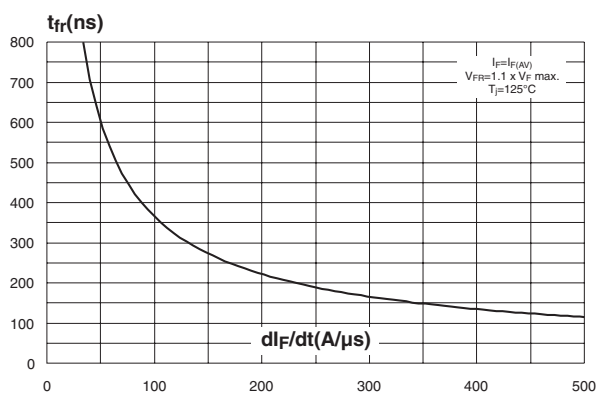
Fig. 10: Forward recovery time versus dl_F/dt (90% confidence).
