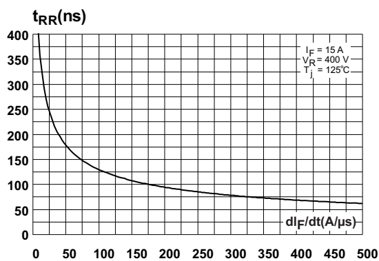
Figure 7. Reverse recovery time versus di_F/dt (typical values, per diode)
