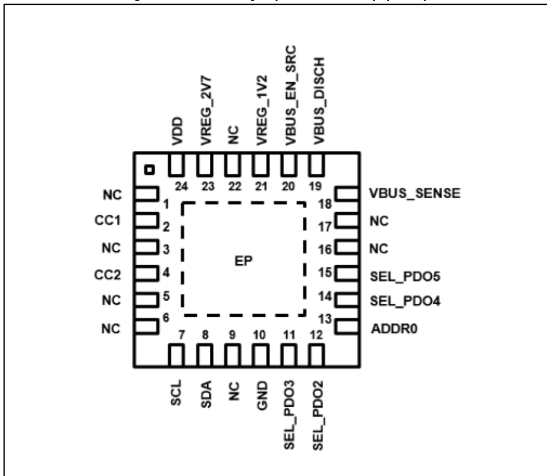
Figure 2: STUSB4710QTR pin connections (top view)
