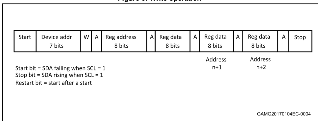
Figure 6: Write operation
