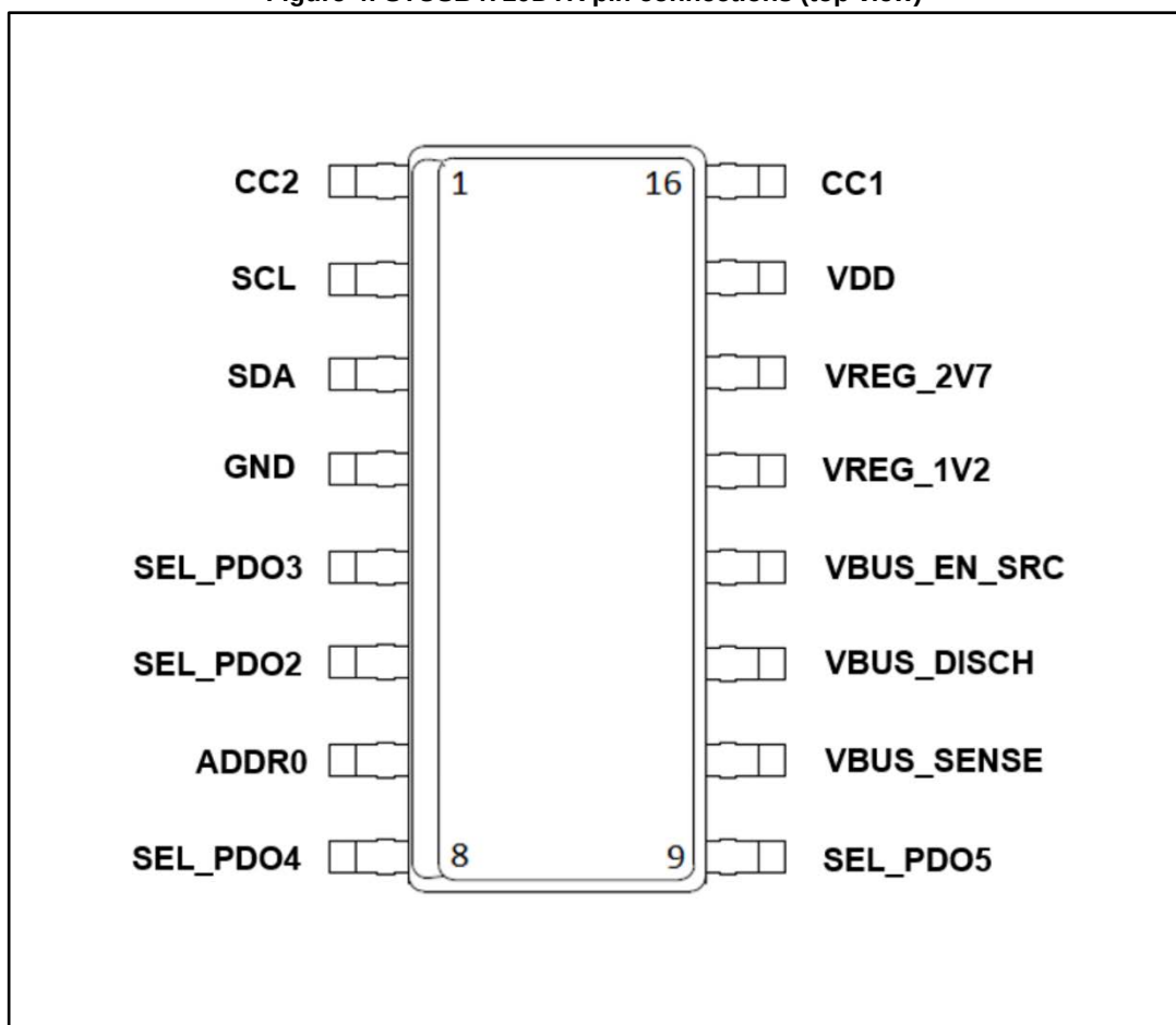
Figure 4: STUSB4710DTR pin connections (top view)
