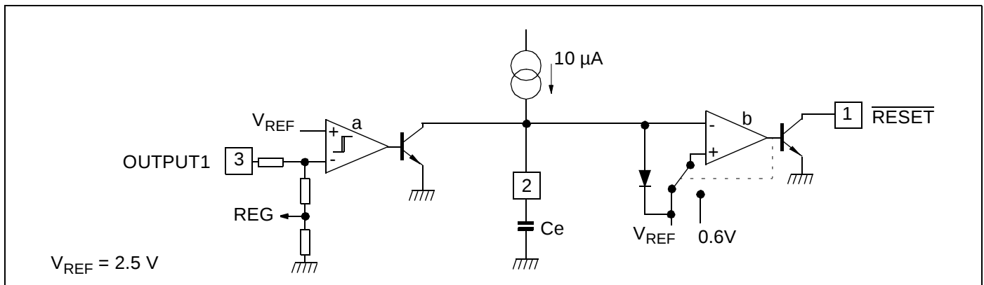
Figure 2: Reset Diagram
