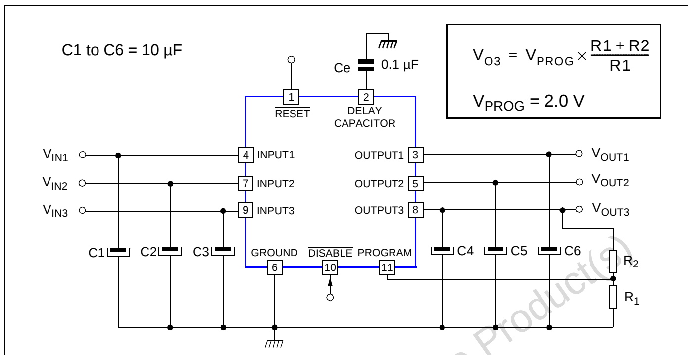
Figure 4: STV8163 Typical Application
