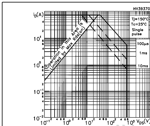
Figure 6. Safe operating area for TO-247
