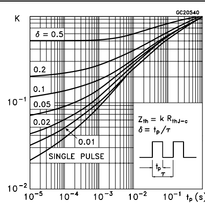
Figure 3. Thermal impedance for TO-220 - D 2 PAK - I 2 PAK
