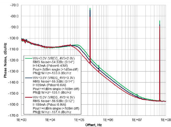
Figure 9. Phase noise and fractional spurs at 2646.96 MHz vs. supply ( F_{\text{PFD}} = 61.44 MHz)
