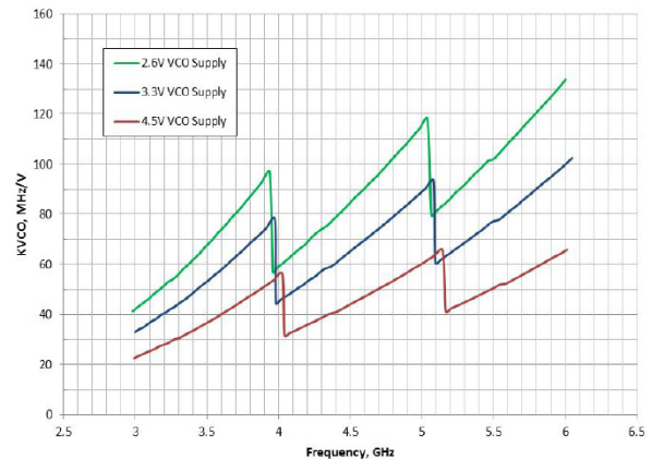
Figure 16. Average K_{\text{VCO}} over VCO frequency and supply
