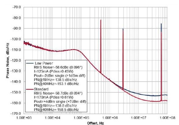
Figure 12. Phase noise and fractional spurs at 2118.24 MHz at 3.6 V supply ( F_{\text{PFD}} = 61.44 MHz)
