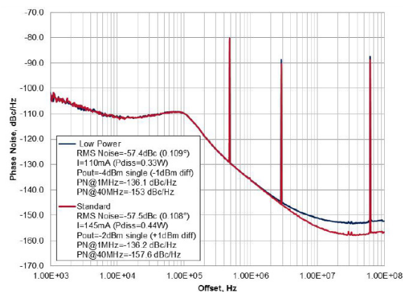
Figure 13. Phase noise and fractional spurs at 2118.24 MHz at 3.0 V supply ( F_{\text{PFD}} = 61.44 \text{ MHz} )
