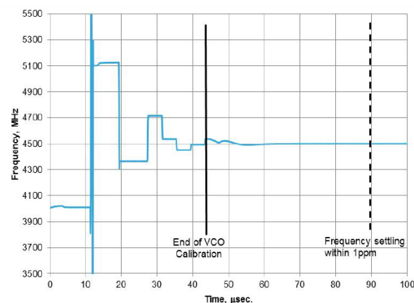
Figure 23. Frequency settling with VCO calibration – wideband view
