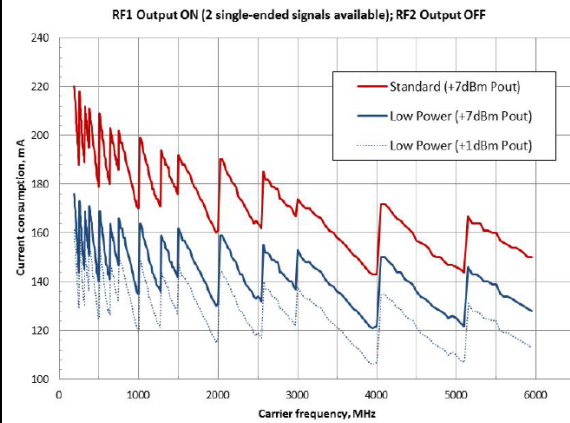
Figure 26. Current consumption – standard vs. low power (5.0 V supply, F_{\text{PFD}} = 50 MHz)
