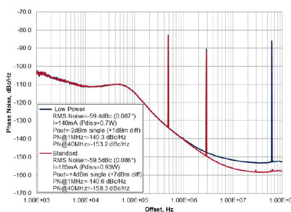
Figure 11. Phase noise and fractional spurs at 2118.24 MHz at 5.0 V supply ( F_{\text{PFD}} = 61.44 MHz)
