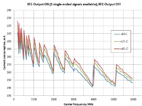
Figure 25. Overall current consumption vs. temperature (5.0 V supply, F_{\text{PFD}} = 50 MHz)
