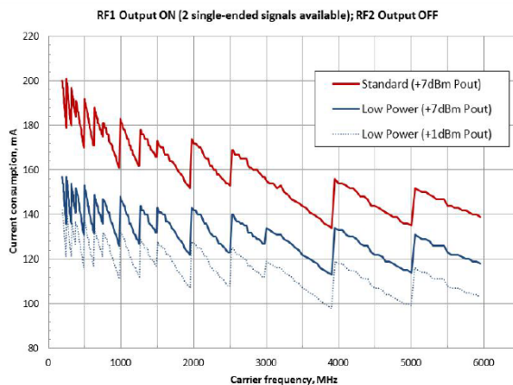
Figure 27. Current consumption – standard vs. low power (3.6 V supply, F_{\text{PFD}} = 50 MHz)
