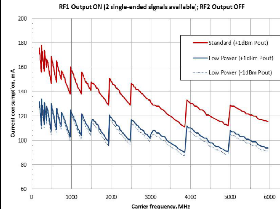
Figure 28. Current consumption – standard vs. low power (3.0 V supply, F_{\text{PFD}} = 50 MHz)
