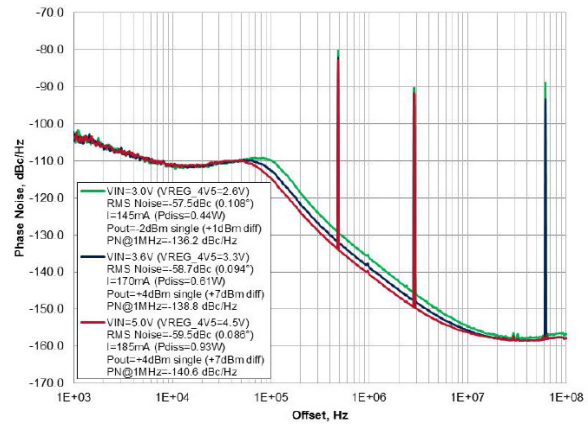
Figure 10. Phase noise and fractional spurs at 2118.24 MHz vs. supply ( F_{\text{PFD}} = 61.44 MHz)
