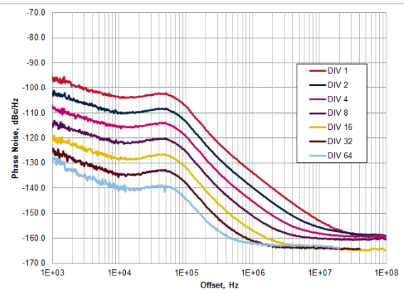
Figure 4. Closed-loop phase noise at 4.8 GHz, divided by 1 to 64 (5 V supply)
