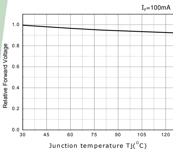
Forward Voltage Shift vs. Junction Temperature
