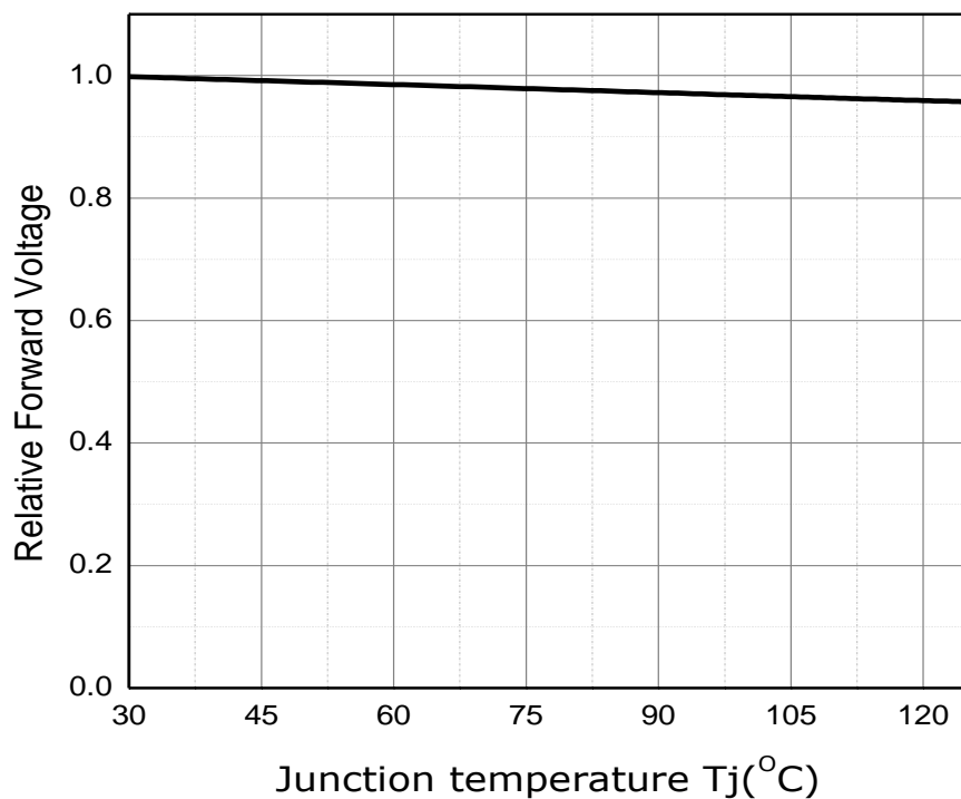
Fig 7. Junction Temperature vs. Relative Forward Voltage
