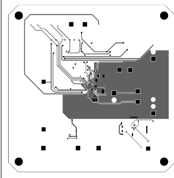
Figure 16: Mid layer 1
