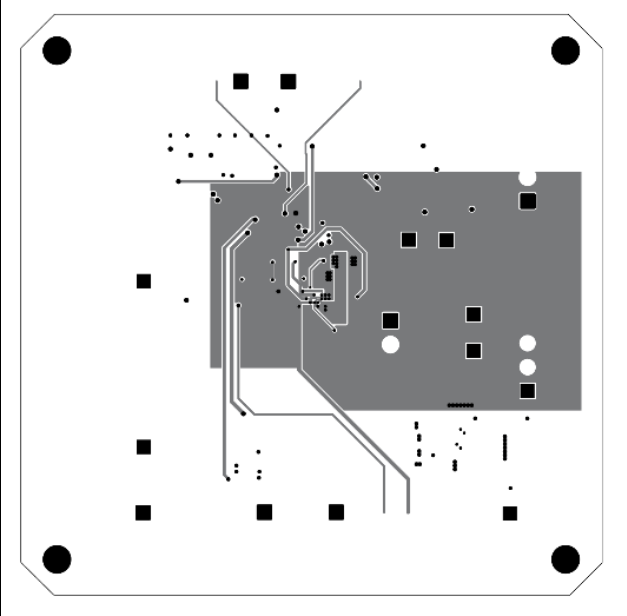
Figure 17: Mid layer 2
