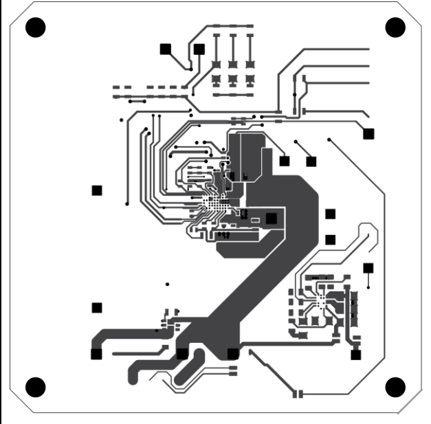
Figure 15: Top layer
