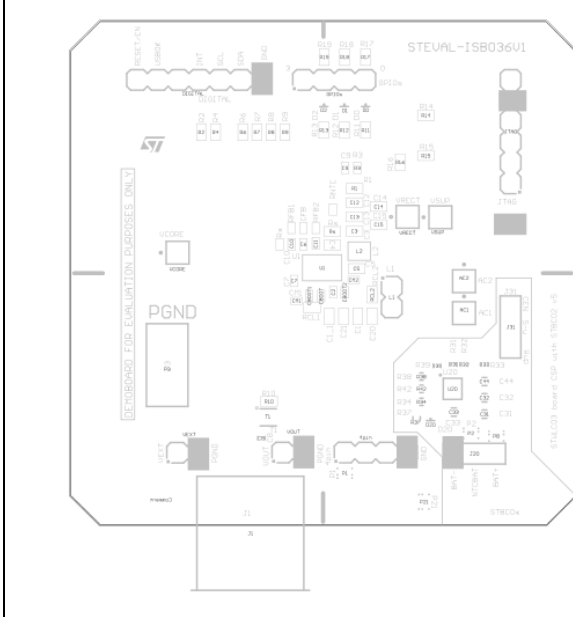
Figure 14: Top overlay
