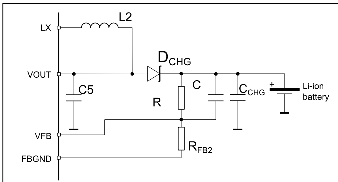
Figure 11: STWLC03 charger configuration
